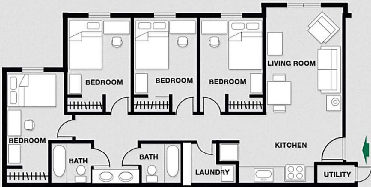
Ground & First Floor Plans
