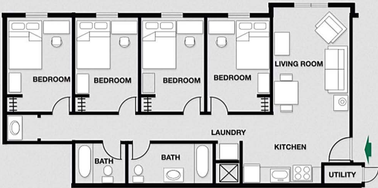
Building 1, First Floor Plans
